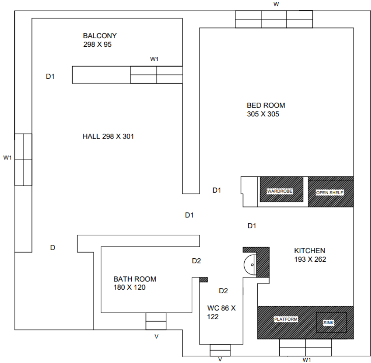
EXISTING LAYOUT OF MEDICAL FLAT - DISMANTLING DETAILS
