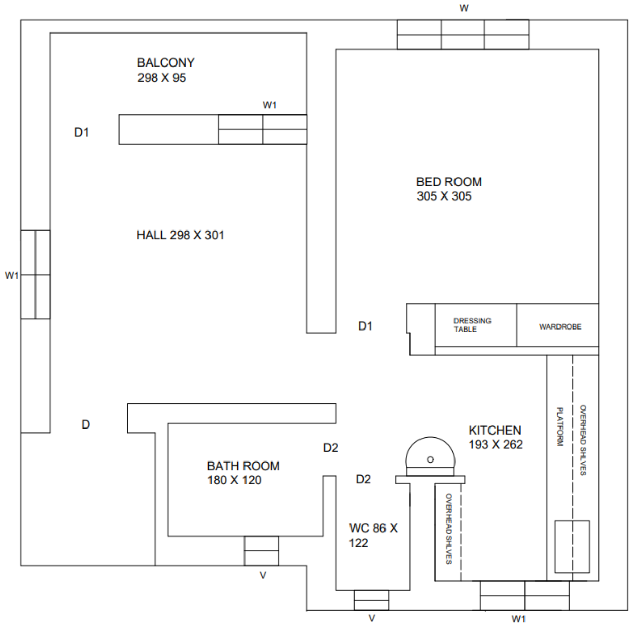
MEDICAL FLAT - PROPOSED LAYOUT
