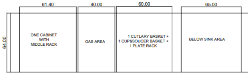
PLAN
