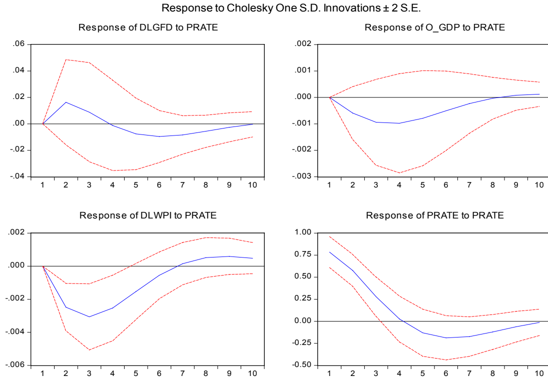
Chart 4: Response to Policy Rate Shock (Corrected)
